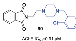
Fig. 34 Structure of phthalimide-piperazine hybrid 60.
