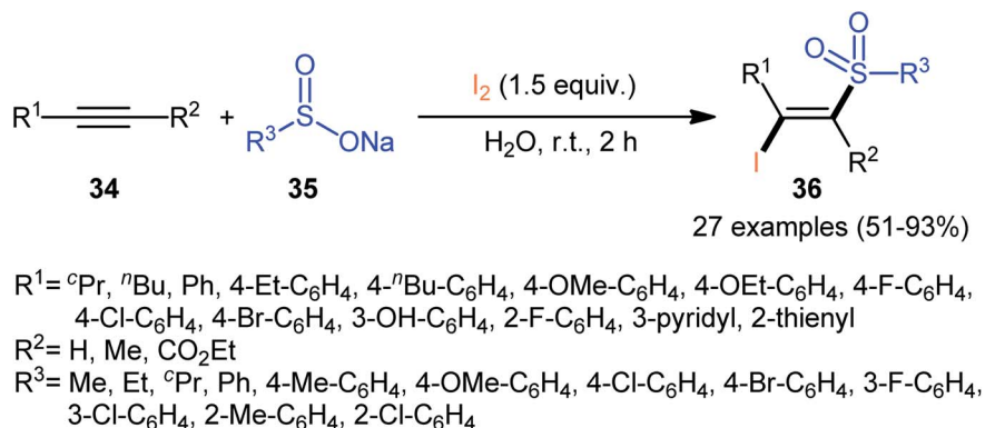
Scheme 15 Catalyst-free synthesis of ( E )-β-iodovinyl sulfones 36 via the reaction of alkynes 34 with sodium sulfonates 35 and I 2 .
