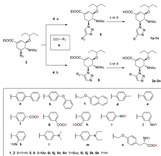
Scheme 1 Synthesis of target compounds. Reagents and conditions: (a) sodium ascorbate, aq CuSO 4 , THF/H 2 O (3 : 1), 45 °C, 6–12 h, 68–98%; (b) Cp*RuCl(PPh 3 ) 2 , THF, 60 °C, 12–24 h, 29–89%; (c) aq NaOH, MeOH, rt, 6–12 h, 55–81%; (d) (i) aq NaOH, MeOH, rt, 6–12 h; (ii) TFA/DCM (1 : 1), rt, 3–4 h, 72–79%.
