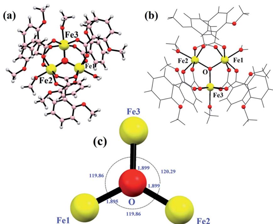
Fig. 2 Ball and stick model (a), wireframe structure (b) and the triangle supported by \mu_3-O (c) in \{Fe_3\} .
