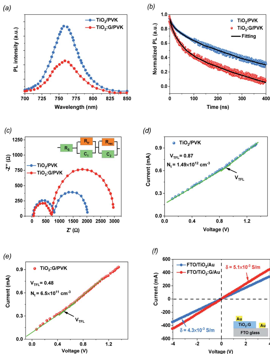
Fig. 4 (a) Steady-state PL spectra. (b) TRPL spectra. (c) Nyquist plots with charge-transfer resistances of 812 Ω and 718 Ω for pure and doped devices, respectively, with the corresponding recombination resistances of 2018 Ω and 2962 Ω. Dark current–voltage curves of the electron-only devices for (d) FTO/TiO 2 /PVK/PCBM/Au and (e) FTO/G:TiO 2 /PVK/PCBM/Au. (f) I – V curves of the devices with an FTO/ETL/Au structure for conductivity measurements.
