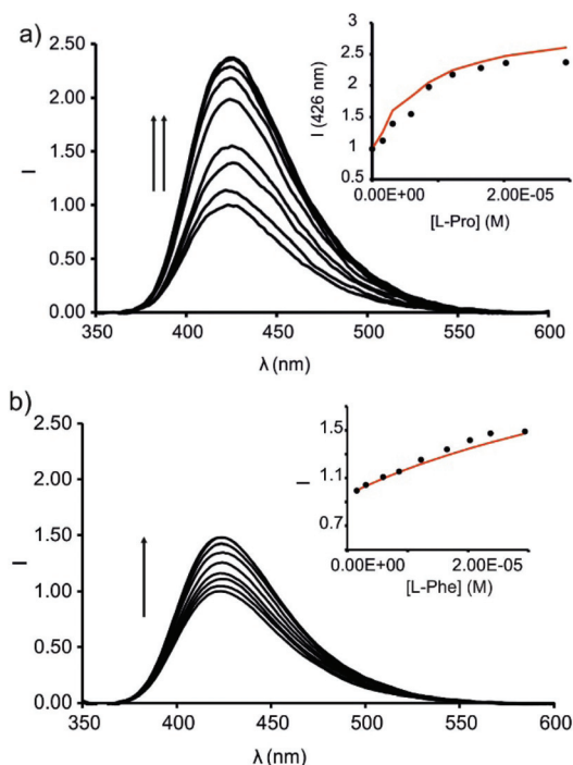
Fig. 9 Emission spectra registered during the competitive IDA experiments of 6-1in complex (1 \mu\text{M} ) with incremental addition of L-Pro (up to 30 equiv.) (a) and L-Phe (up to 30 equiv.) (b) in dichloromethane solution; \lambda_{\text{exc}} = 335 \text{ nm} . Insets: plots of the emission change at 426 nm (black circles) vs. concentration of the amino acid. The red line corresponds to the fit of the titration data to a 1:1 theoretical binding model considering only two emissive species: the free cavitand and the 1:1 complex with the corresponding amino acid.
