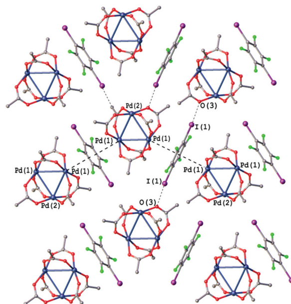
Fig. 8 Crystal structure diagram of [Pd 3 ](1,4-IFB). Selected distances (Å): I(1)...O(3) 3.399, Pd(1)...(1,4-IFB) centroid 3.349. Short I...O contacts and PdO 4 ... \pi interactions are clearly seen in the Hirshfeld surface map (Fig. S5†).
