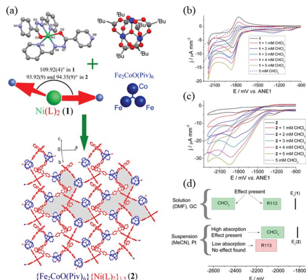
Fig. 7 A \text{Fe}^{\text{III}}\text{--Ni}^{\text{II}} bimetallic coordination polymer as a dehalogenation electrocatalyst: (a) synthesis scheme and structures, (b) CV curves of the \text{Ni}^{\text{II}} metalloligand in DMF with the addition of \text{CHCl}_3 , (c) CV curves of the suspension containing the \text{Fe}^{\text{III}}\text{--Ni}^{\text{II}} bimetallic coordination polymer in \text{CH}_3\text{CN} with the addition of \text{CHCl}_3 , and (d) catalytic activities vs. redox potentials of the catalysts and the halides. Adapted with permission from ref. 102, Copyright 2014 American Chemical Society.
