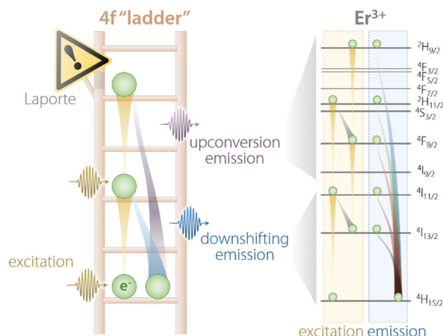
Fig. 1 Schematic representation of the “4f ladder” featured by \text{Ln}^{3+} ions, along with the real example of \text{Er}^{3+} excitation and emission processes under 980 nm excitation.
