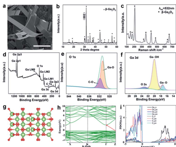
Fig. 4 Characterization of \beta -Ga 2 O 3 nanobelts. (a) SEM image of hexagonal \beta -Ga 2 O 3 nanobelts. (b) XRD spectrum of \beta -Ga 2 O 3 . (c) Raman spectrum of the \beta -Ga 2 O 3 crystal. (d–f) XPS results of \beta -Ga 2 O 3 nanobelts. (g) Crystal structure of \beta -Ga 2 O 3 . (h) Band structure of \beta -Ga 2 O 3 . The Fermi energy is aligned to zero. (i) PDOS of \beta -Ga 2 O 3 . The scale bar in (a) is 10 \mu\text{m} .
