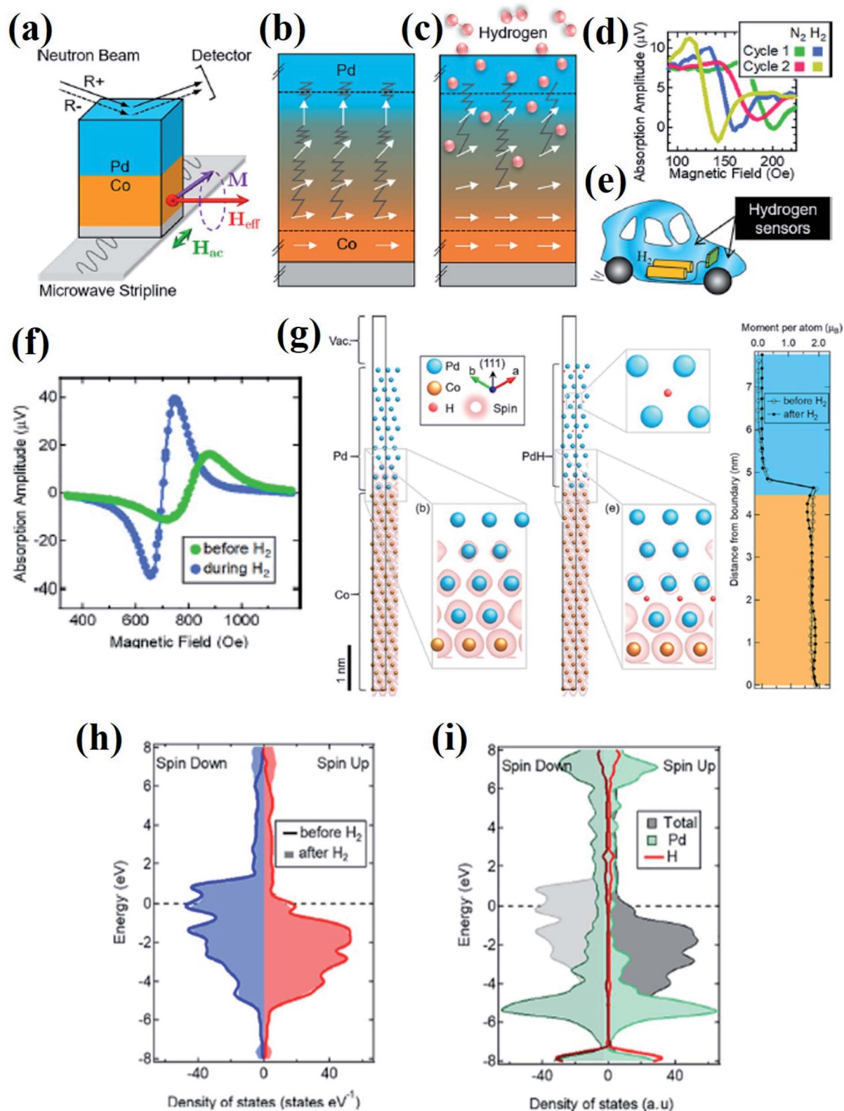
Fig. 11 In operando study of the FMR based hydrogen sensing using Co/Pd film. (a) Polarized neutron reflectometry (PNR) with an in situ FMR experimental setup (b) before and (c) during exposure to \text{H}_2 gas demonstrating the modification of Co/Pd interface with the change in the projection of the FM spins into the film plane. (d) FMR spectra of a Co (5 nm)/Pd (15 nm) film displaying excellent cycling ability between the first and second consecutive exposures to hydrogen gas. (e) Schematic illustration of the application of \text{H}_2 sensor in hydrogen fuel cell vehicle. (f) Field-resolved FMR spectra of the Co/Pd film during hydrogen gas cycling. (g) DFT calculations of the theoretical Co/Pd thin-film structure. Electronic density of states determined from DFT calculations for a theoretical Co/Pd thin-film structure. (h) Total spin-resolved density of states and (i) site-projected density of states, including the projected density of states contributed by a hydrogen and a Pd site. Reprinted with permission from ref. 83. Copyright (2019) American Chemical Society.
