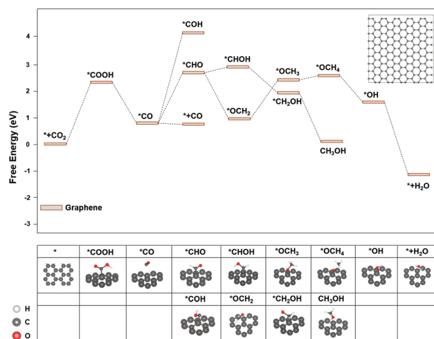
Fig. 3 The free energy diagram of CO_2RR on graphene. Noted that *OCOH could not form a stable adsorption structure on graphene. Inset: The graphene model used for the calculations.
