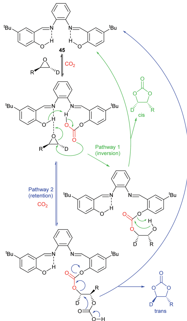
Scheme 21 Proposed mechanisms for cyclic carbonate formation using salphen 45.
