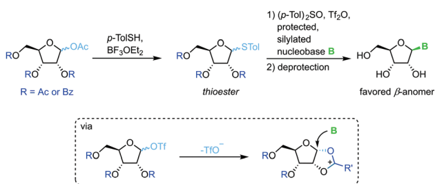
Scheme 11 Nucleobase glycosylation with thioglycosides.
