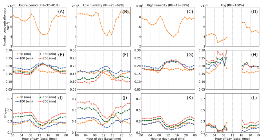
Fig. 8 Diel variations of particle number concentration in PM_{10} size range (top row), hygroscopicity parameter \kappa (second row) and number fraction of hydrophobic particles Nf_{\text{hydro}} for selected particle sizes (bottom row) averaged over the entire campaign and focus periods with different relative humidity (RH) conditions.
