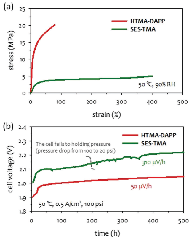
Fig. 16 (a) Stress–strain curves of HTMA-DAPP and SES-TMA AEMs. (b) Comparison of long-term performance of AEMWEs using HTMA-DAPP (78 μm thick) and SES-TMA (53 μm thick) AEMs. Ionomer: Aemion, Co 3 O 4 (3 mg cm -2 ), cathode: Pt black (3 mg Pt cm -2 ). The AEMWE cell data was produced at Nel Hydrogen.
