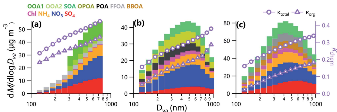
Fig. 7 Average size distributions of \kappa_{\text{chem}} and \kappa_{\text{org}} , and the contributions of NR-PM 1 species (SO 4 , NO 3 , NH 4 , Chl, and OA factors) in (a) summer and (b) winter in Beijing, and (c) winter in Gucheng.
