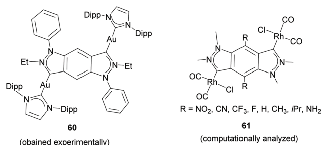
Scheme 19 Dimetallic complexes with a benzo-fused bis-pyrazolyldene.
