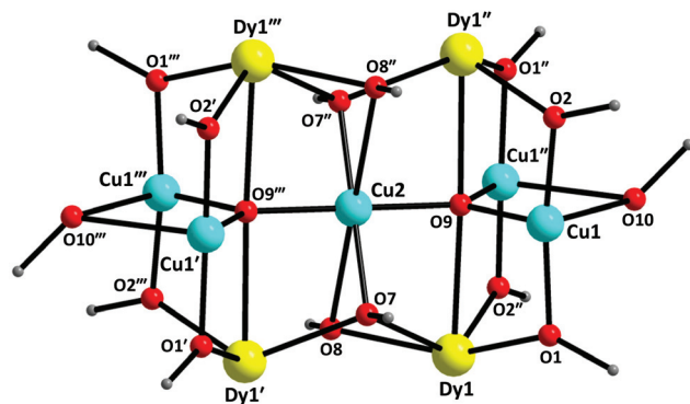
Fig. 2 The \{Cu_5Dy_4(\mu_5-O)_2(\mu_3-OMeO)_4(\mu-OMeOH)_2(\mu-OR')_8\}^{6+} core of the cluster molecule 1 . O9, O9''' represent the \mu_5 -oxo groups; O7, O7'', O8, O8'' are the \mu_3 -methoxo oxygen atoms; O10, O10''' denote the bridging methanol oxygen atoms; O1, O2 and their symmetry equivalents belong to the pdm^{2-} ligands. The symmetry codes are the same with those defined in the caption of Fig. 1.
