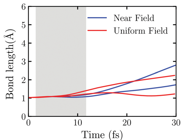
Fig. 6 Time evolution of the OH bonds of \text{Au}_{20}@\text{H}_2\text{O} interacting with the real near field and the uniform electric field, respectively. Here the laser field with E_{\text{max}}^0 = 0.65 \text{ V } \text{\AA}^{-1} and \omega_0 = 3.07 \text{ eV} is applied.
