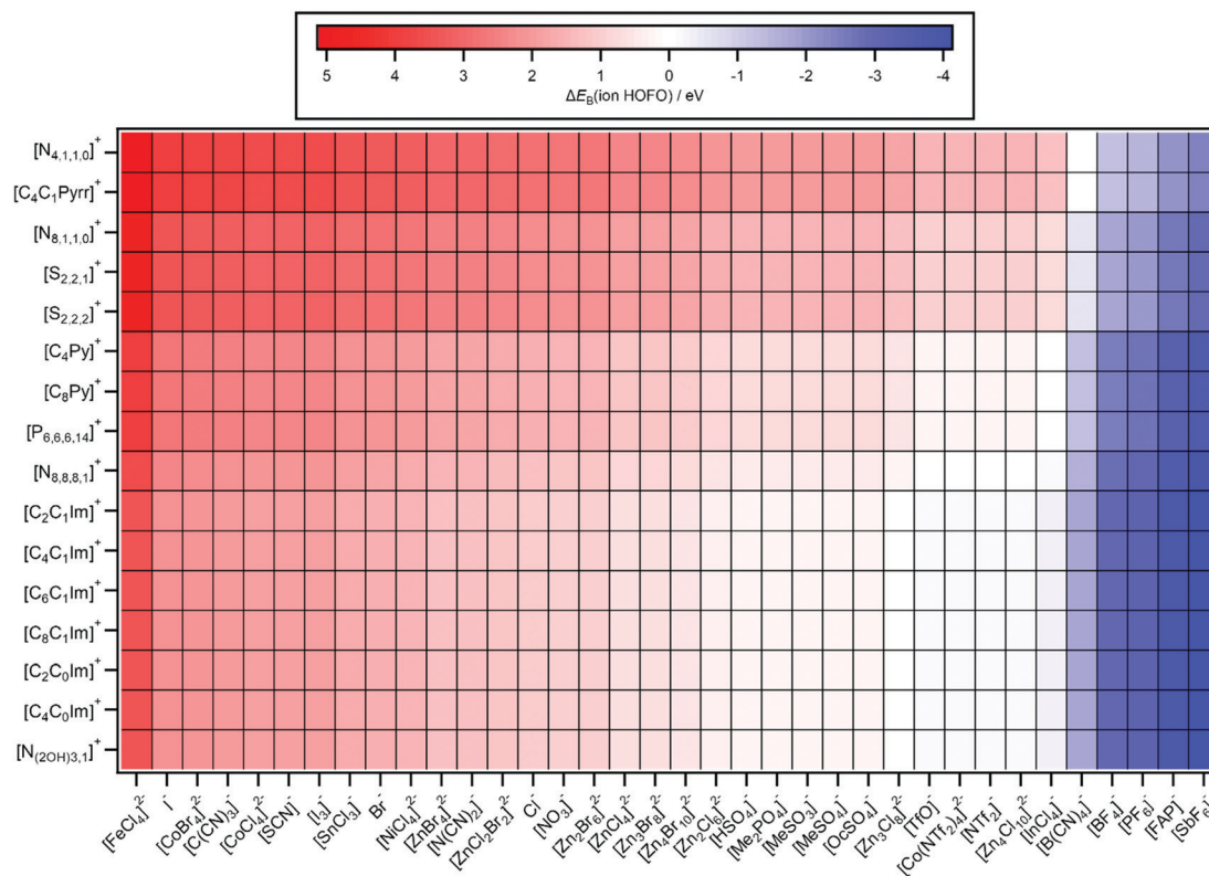
Fig. 7 Predicted \Delta E_B(\text{ion HOFO, pred.}) = E_B(\text{cation HOFO, pred.}) - E_B(\text{anion HOFO, pred.}) = E_i(\text{cation, pred.}) - E_i(\text{anion, pred.}) . The errors in \Delta E_B(\text{ion HOFO, pred.}) generally range from \pm 0.4 eV to \pm 0.6 eV.
