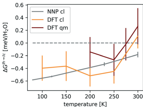
Fig. 4 \Delta G^{\text{Ih}-\text{Ic}}(T) with error bars at ambient pressure. The errors associated with the classical (cl) and quantum-mechanical (qm) revPBE0-D3 values arise predominantly from differences in \Delta G_{\text{NNP}} between proton-orderings. The smaller errors in \Delta G_{\text{cl,NNP}}^{\text{Ih}-\text{Ic}}(T) are due to the larger simulation cell used to obtain it. The data was taken from ref. 115.
