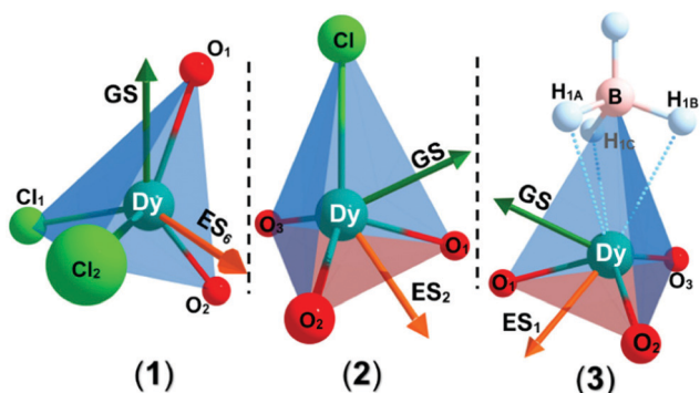
Fig. 2 Local coordination environments of 1–3 (Dy teal, Cl green, O red, B pink, H pale blue). Arrows represent CASSCF-SO calculated magnetic axis ( g_2 vector), GS (dark green), and selected ES (orange) with significant angles of deviation of the g_2 vector from the GS.
