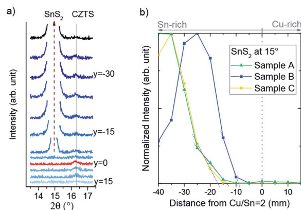
Fig. 3 (a) XRD patterns in regions with \text{SnS}_2 reflection at 15^\circ for different positions parallel to the \text{Cu}/\text{Sn} = 2 line on sample B. y denotes the distance to the \text{Cu}/\text{Sn} = 2 line in mm. (b) Integrated intensity of the reflection at 15^\circ . The dotted lines are guides to the eye for the interpolation to the phase boundary.
