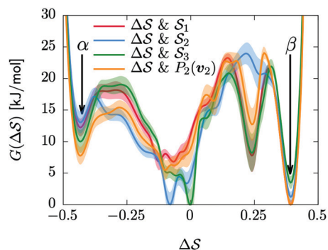
Fig. 3 Convergence of the free-energy calculations. Comparison of four metadynamics simulations at T = 400 \text{ K} with different CVs (see labels) projected on \Delta S .
