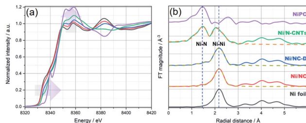
Fig. 3 (a) Normalized XANES spectra and (b) Fourier transform (FT) of k^2 -weighted EXAFS spectra and the fit results (dashed lines) for Ni foil (black), Ni/NC (red), Ni/NC-D (blue), Ni/N-CNTs (green), and Ni-Pc (purple), respectively. The blue vertical dashed lines at ca. 1.45 and 2.19 Å in (b) are to mark the position of Ni–N and Ni–Ni bonds, respectively. Details on the EXAFS analysis are provided in the ESI.†
