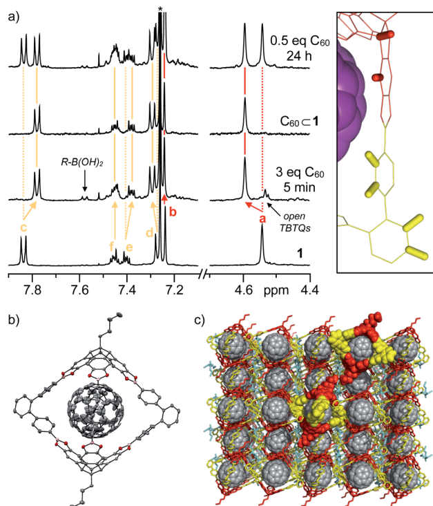
Fig. 3 (a) ^1\text{H} -NMR spectra (400 MHz, \text{CDCl}_3 , rt) for complexation of 1 with \text{C}_{60} , (b) ORTEP representation of single-crystal X-ray structure of \text{C}_{60}\text{C}1 (thermal ellipsoids were set at 50% probability, C = grey, O = red, B = purple, H atoms were omitted for clarity) and (c) packing of \text{C}_{60}\text{C}1 in the solid state indicating the accessible \text{C}_{60} surface in the three cage windows.
