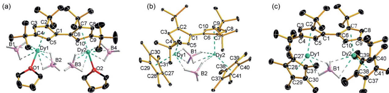
Fig. 1 Thermal ellipsoid representations (30% probability) of the structures of: (a) 1, (b) 2 and (c) 3. For clarity, hydrogen atoms are omitted except those in the [\text{B}(\text{H}_4)]^- ligands.
