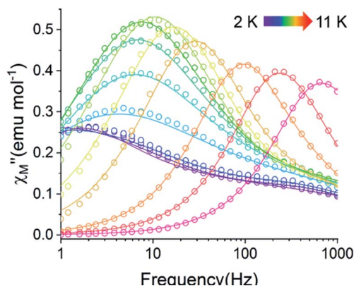
Fig. 9 Temperature dependence of the out-of-phase component of the molar ac magnetic susceptibility ( \chi''_{\text{M}} ) of 2 at 0.35 T ( H = 0.35 T , T = 2 – 11 K). Lines represent fits to the experimental data (circles).
