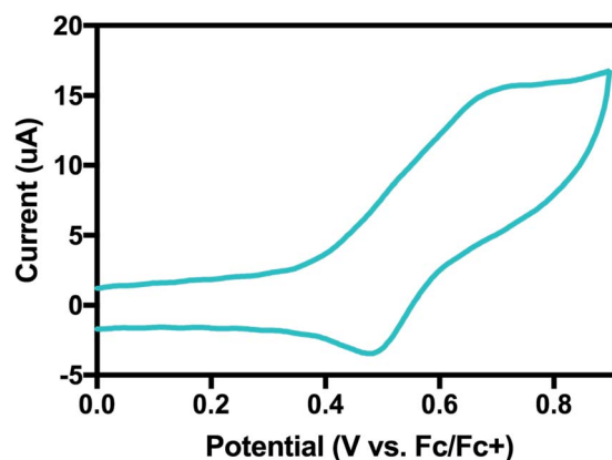
Fig. 10 Cyclic voltammogram of 4 in MeCN. The quasi-reversible couple at E^0 = 0.58 \text{ V} vs. \text{Fc}/\text{Fc}^+ is assigned as a \text{Ni}(\text{II}/\text{III}) couple.
