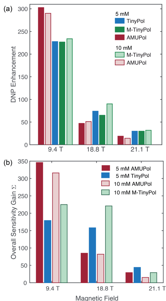
Fig. 4 DNP enhancement factors (a) and overall sensitivity gains (b) of 5 mM and 10 mM TinyPol, M-TinyPol and AMUPol solutions in d_8 -glycerol/ D_2O/H_2O 60/30/10 (v/v/v) acquired at various magnetic fields. Data recorded at 9.4 T and 18.8 T were acquired in 1.3 mm zirconia rotors at 40 kHz MAS frequency and a sample temperature of \sim 110 K. Data recorded at 21.1 T were acquired in 3.2 mm sapphire rotors at 12 kHz MAS frequency and a sample temperature of \sim 115 K. The calculation of \Sigma is given in the ESI.†
