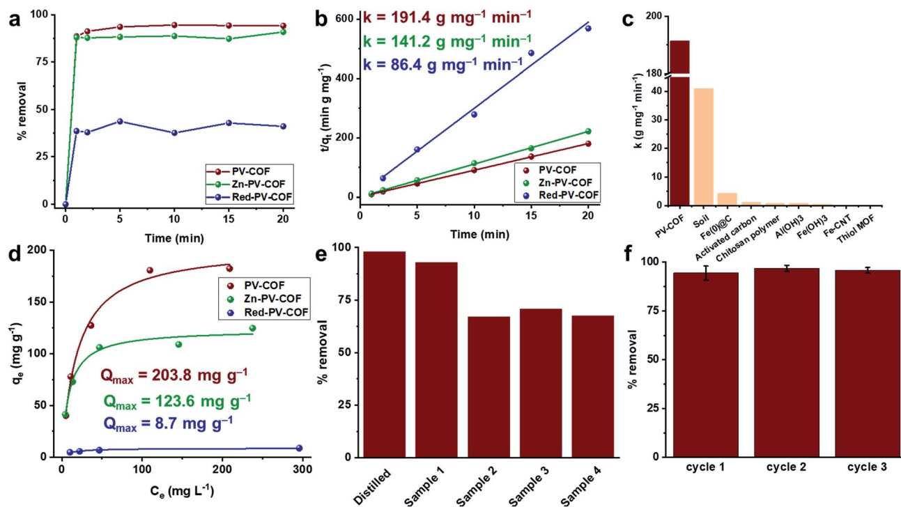
Fig. 4 Bromate adsorption results. (a) % removal of BrO_3^- by PV-COF, Zn-PV-COF and Red-PV-COF with 50 \mu g L^{-1} initial concentration of BrO_3^- at different time points ( n = 3 ); (b) the pseudo-second-order kinetic plots for BrO_3^- adsorption by PV-COF, Zn-PV-COF and Red-PV-COF along with associated rate constants ( k ); (c) a comparison of the rate constants of PV-COF and other reported bromate adsorbents; (d) Langmuir non-linear isotherm model fitting for PV-COF, Zn-PV-COF and Red-PV-COF along with determined maximum adsorption capacities ( Q_{max} ) at BrO_3^- concentrations in the range 12.5 – 200 mg L^{-1} ; (e) % removal of BrO_3^- after 20 min incubation of PV-COF with commercial water samples from the UAE, Italy and Norway to which BrO_3^- was added at a concentration of 50 \mu g L^{-1} . Water samples contained competitive anions, including bicarbonate ( 0 – 182 mg L^{-1} ), sulfate ( 0 – 86 mg L^{-1} ), chloride ( 1.3 – 77 mg L^{-1} ), nitrate ( 0.3 – 1.1 mg L^{-1} ) and fluoride ( 0.1 – 0.5 mg L^{-1} ); (f) regeneration efficiency of PV-COF for BrO_3^- adsorption; uptake efficiency is preserved for at least three cycles.
