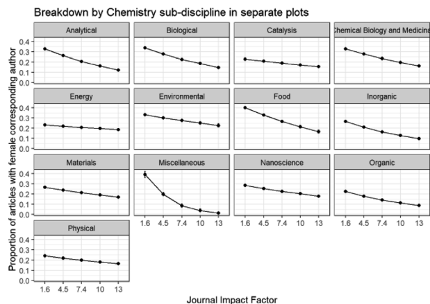
Fig. 22 Binomial GLM model of corresponding author gender of accepted submissions, chemistry sub-discipline and journal impact factor (Model: CorrAuthorGender \sim Category * ImpactFactor). ANOVA \text{Pr}(>\text{Chi}) : Category is highly significant ( 0.00 \times 10^0 ); ImpactFactor is highly significant ( 0.00 \times 10^0 ); Category: ImpactFactor interactions are highly significant ( 3.18 \times 10^{-73} ).
