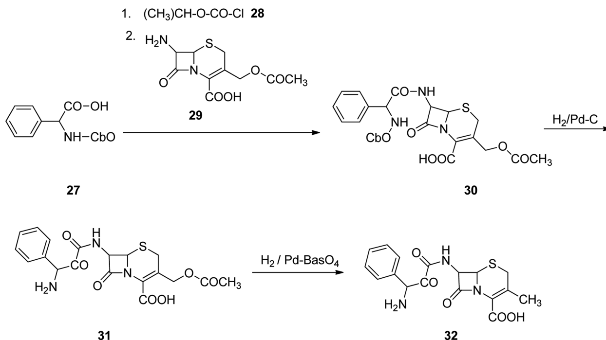
Scheme 4 Synthesis of cephalaxin 32 .
