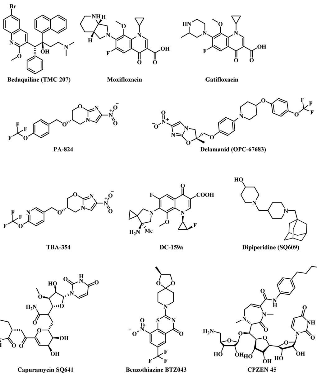
Fig. 1 Various antitubercular compounds.
