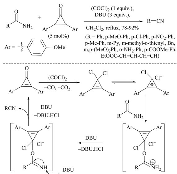
Scheme 52 Organocatalytic dehydration.
