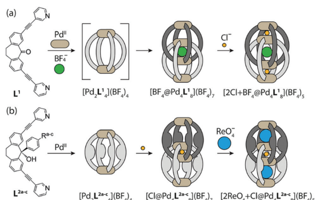
Fig. 16 Synthesis of interpenetrated dimer cage: (a) [\text{Pd}_4\text{L}_8\text{-BF}_4] with \text{BF}_4^- as a template anion and \text{Cl}^- anions in the outer pockets, (b) [\text{Pd}_4\text{L}_8\text{-Cl}] with \text{Cl}^- as a template anion and \text{ReO}_4^- in the outer pockets. Reproduced with permission from ref. 73. Copyright 2013, American Chemical Society.
