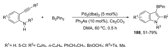
Scheme 154
