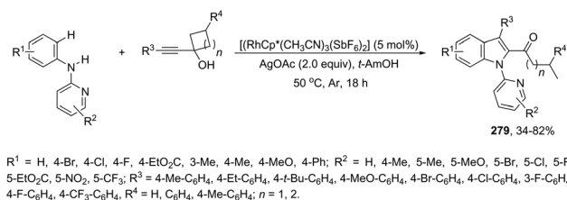
Scheme 223
