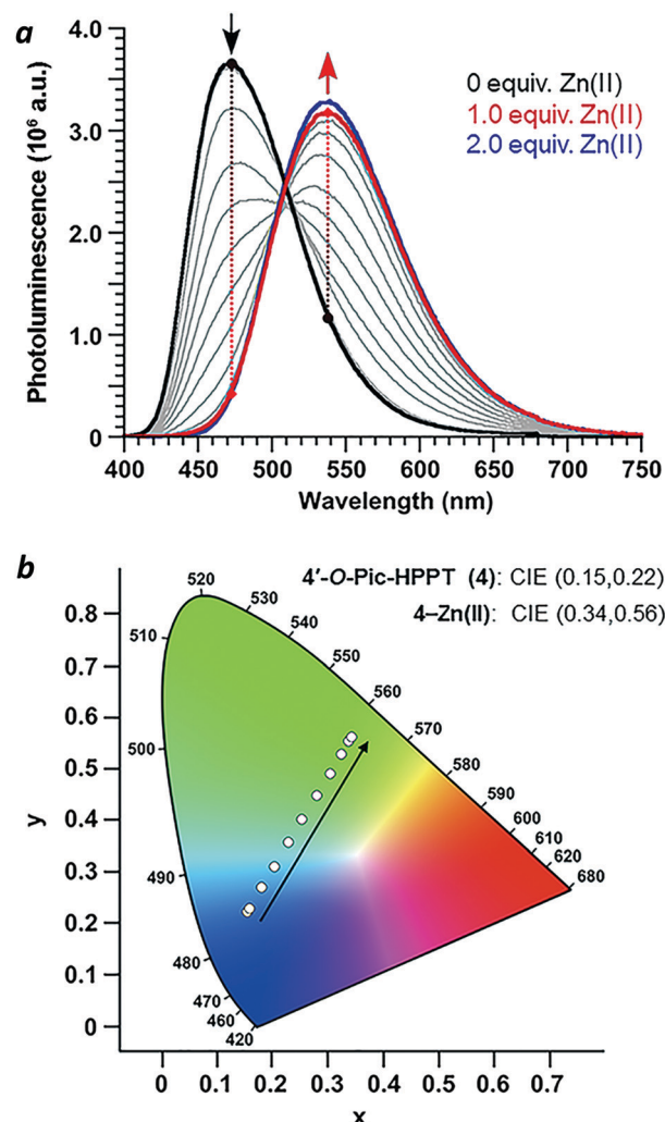
Fig. 6 (a) Spectral changes in the photoluminescence of 4 (30 μM in CH 3 CN) upon titration of Zn(NO 3 ) 2 ·6H 2 O (3 mM in CH 3 CN) and excitation at the isosbestic point ( \lambda_{\text{ex}} = 393 nm). (b) CIE chromaticity diagram of 4 showing the progression in emitted light with Zn(II) addition.
