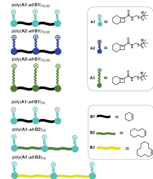
Fig. 1 Structures of monomers (before ring-opening) and polymers synthesized and characterized in this work.
