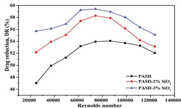
Fig. 14 Drag reduction as a function of Reynolds number.
