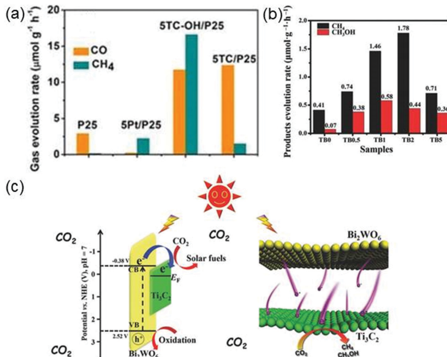
Fig. 12 (a) Evolution rates of CO and CH 4 over P25, 5Pt/P25 (containing 5 wt% Pt), 5Ti 3 C 2 T x /P25 (containing 5 wt% Ti 3 C 2 T x ) and 5TCOH/P25 (containing 5 wt% Ti 3 C 2 T x -OH) under the irradiation of a 300 W Xe lamp. Reprinted with permission from ref. 36 Copyright (2018) Wiley Online Library. (b) Photocatalytic activity (products evolution rates) of Ti 3 C 2 T x -Bi 2 WO 6 (TB) with different weights of Ti 3 C 2 T x (0, 0.5, 1, 2 and 5 wt%). (c) Energy level structure of the TB hybrid (left panel) and the photo-induced electron transfer process at the TB interface (right panel). Reprinted with permission from ref. 158 Copyright (2018) Advanced Science News.
