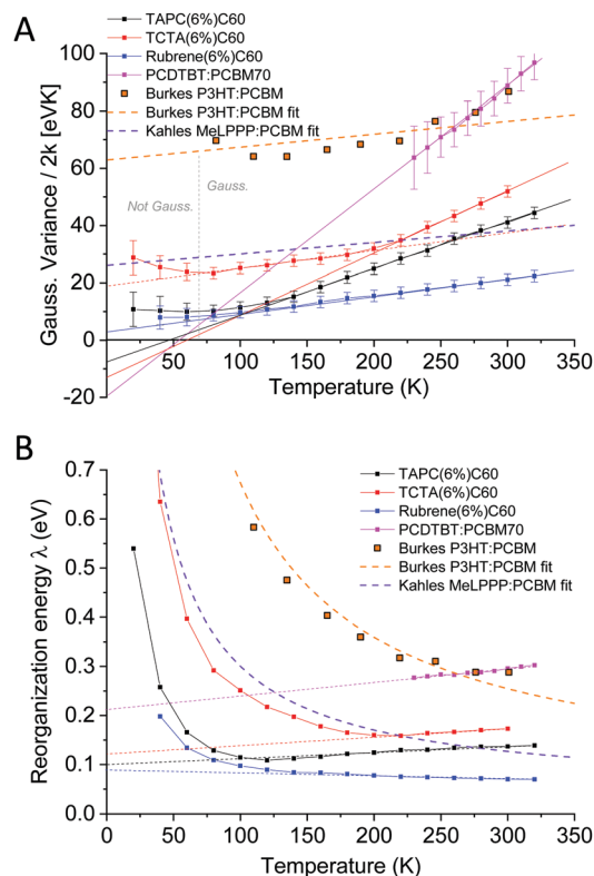
Fig. 8 (A) Temperature dependence of the obtained Gaussian variance of the E^3 reduced spectra from the electroluminescence in Fig. 6. (B) The corresponding “apparent” reorganization energy, determined by dividing the data in (A) with the temperature. Whereas Burke’s EQE and Kahle’s PL data showed strongly T -dependent reorganization energies (almost constant variance dominated by static disorder) our data do not indicate any pronounced contribution to line-width broadening from static disorder.
