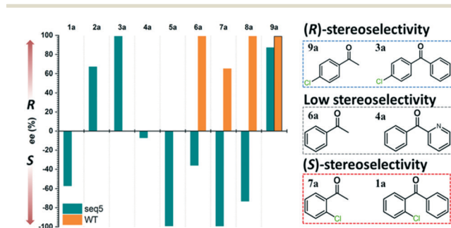
Fig. 5 Stereoselectivities of seq5 for different substituted ketones. The chlorine position plays an important role in product stereo configuration.
