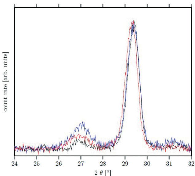
Fig. 8 XRD data of NaSrGdF 6 /β-Na 1.125 Sr 0.75 Gd 1.125 F 6 core/shell particles after heating at 320 °C for 90 min (black), 200 min (red) and 720 min (blue). The peak at \approx 27^\circ belonging to the \alpha -phase is much less intense than the signal of the \beta -phase at \approx 29.5^\circ (compare also with Fig. 2).
