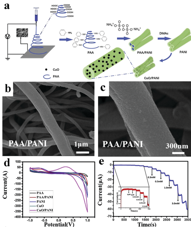
Fig. 6 (a) Schematic diagram of CuO/PANI nano-hybrid fiber synthesis. (b) Low magnification SEM image of the PAA hybrid nanofiber covered by PANI. (c) High magnification SEM image of the PAA hybrid nanofiber covered by PANI. (d) CV curves of GCEs modified with CuO/PANI nano-hybrid fibers. (e) Amperometric response of GCEs modified with CuO/PANI nano-hybrid fibers. Reproduced ref. 48 with permission from Elsevier B.V., copyright 2019.
