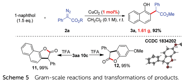
Scheme 5 Gram-scale reactions and transformations of products.
