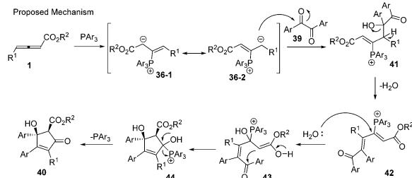
Scheme 12 Phosphine-mediated reaction of \gamma -alkyl allenates and diaryl 1,2-diones.
