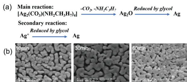
Fig. 14 (a) Two main reaction mechanisms of the silver carbonate–amide complex ink during sintering; (b) SEM images of the conductive film sintered for 10, 30 and 60 minutes. Reproduced with permission from ref. 47. Copyright 2012, Royal Society of Chemistry.
