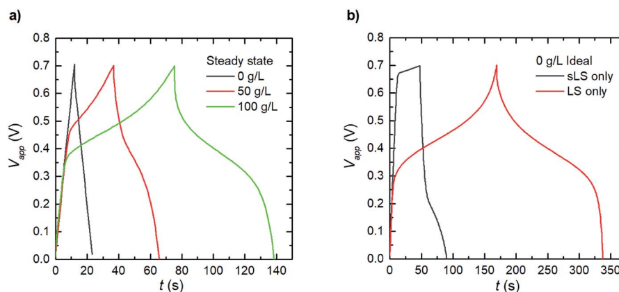
Fig. 5 Simulated electrode response under galvanostatic charge–discharge at 1689 \mu A (2 A g -1 ) for 1_2 electrodes. (a) At steady operation (after long cycling), and (b) for idealized cases where LS is confined in electrode domain in only solid (sLS) or dissolved (LS) form.
